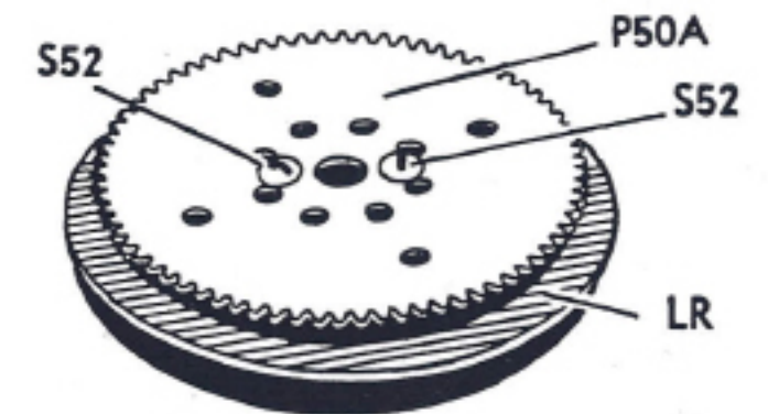
Drive Gear and Drive Wheel Assembly
