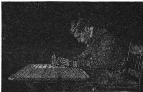
Fig. 103. You light the match in the bottle
