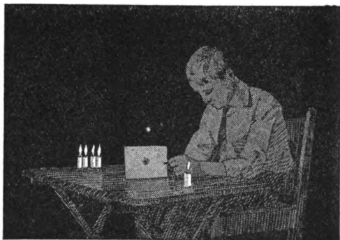
Fig. 30. One candle at one foot is equal to four at two feet
