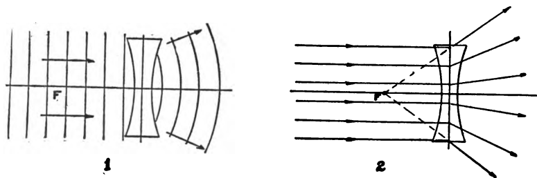
Fig. 163. Parallel waves and rays are diverged
