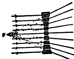
Fig. 156 (1). A converging lens as sections of prisms From Lynde's Physics of the Household , published by The Macmillan Co.
