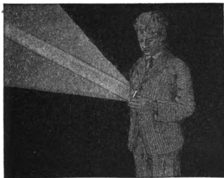
Fig. 98. You see the light spread K — 5
