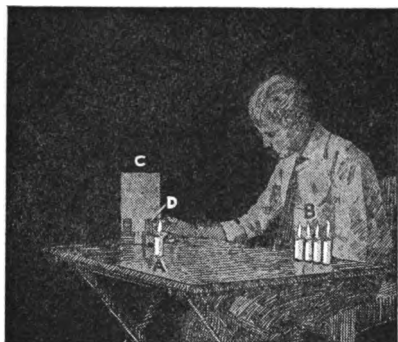
Fig. 33. One candle equal to four From Millikan and Gale's First Course in Physics , Ginn & Co.
