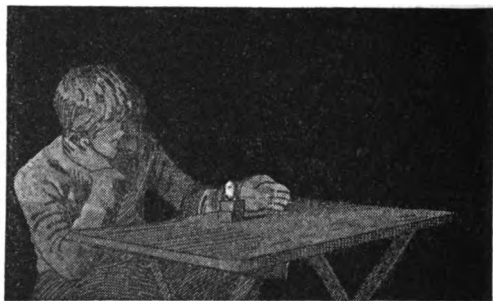
Fig. 159. The focus is hot
