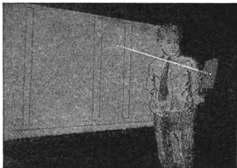
Fig. 9. You see one image of the sun
