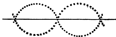
Fig. 143. The waves destroy each other or interfere
