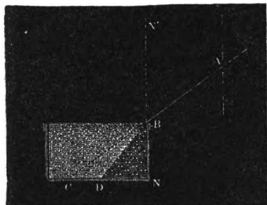
Fig. 111. The light is bent or refracted From Lynde's Physics of the Household , published by The Macmillan Co.
