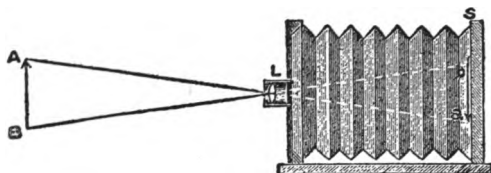
Fig. 183. A camera
