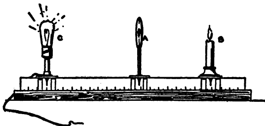
Fig. 32. Bunsen's photometer
