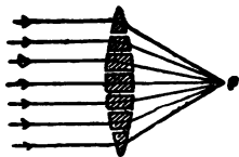
Fig. 156 (1). A converging lens as sections of prisms From Lynde's Physics of the Household , published by The Macmillan Co.
