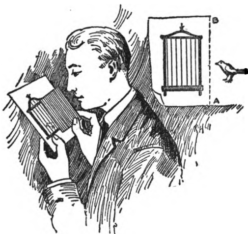
Fig. 192. To make the bird enter the cage
