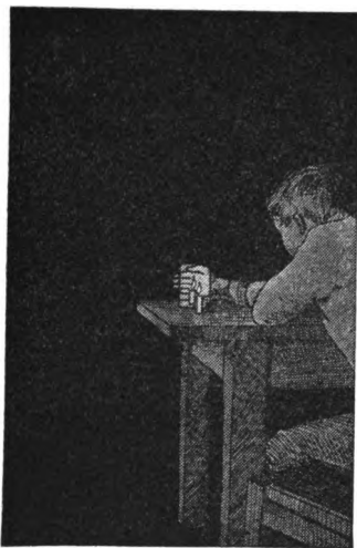
Fig. 67. The candle appears to burn in your hand
