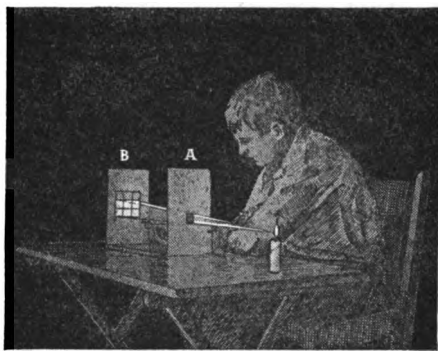
Fig. 27. The light is one-ninth as strong on B as on A when B is 3 feet from the candle
